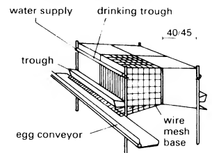
⑧ Battery system, three tiers, about 4800 birds
